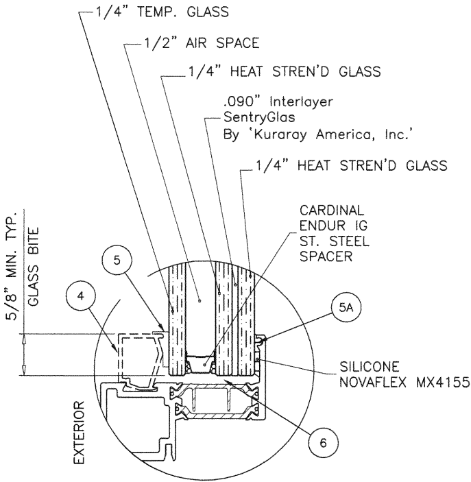
GLAZING DETAIL 1-1/4" OVERALL INSUL. LAM. GLASS
